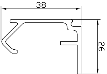
21A Top Track Aluminium
