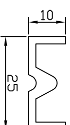
918 Bottom Rail Brass
