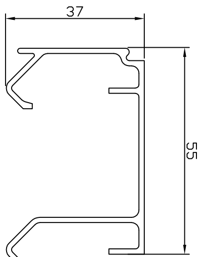
20A Top Track Aluminium
