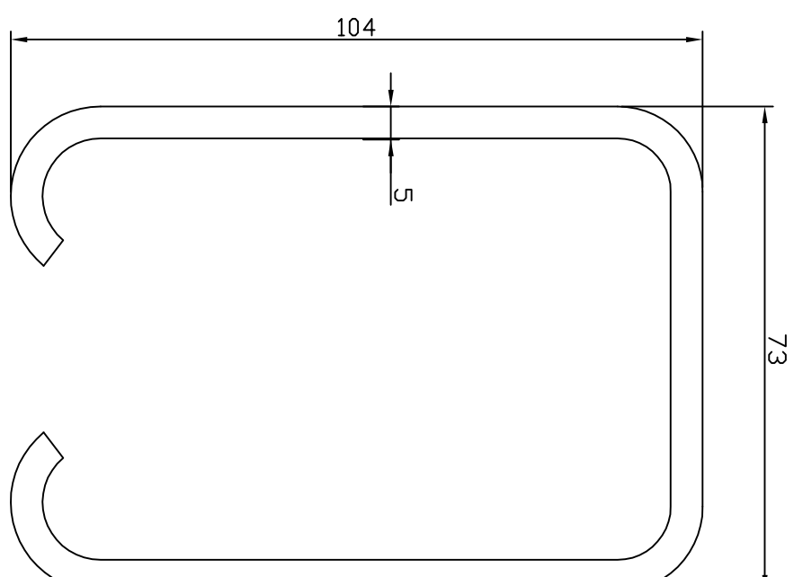
307 Top Track Zinc Plated Steel
