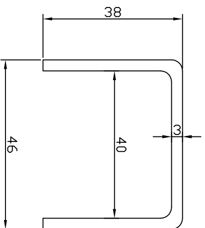
99 Top Guide Channel Steel
