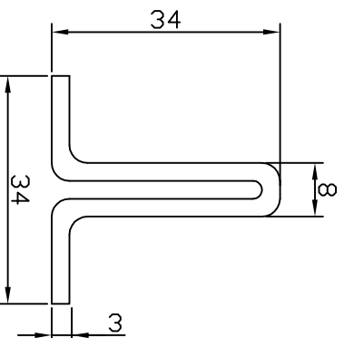
298 Bottom Rail Steel
