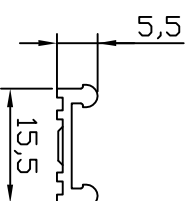
510 Bottom Rail Aluminum
