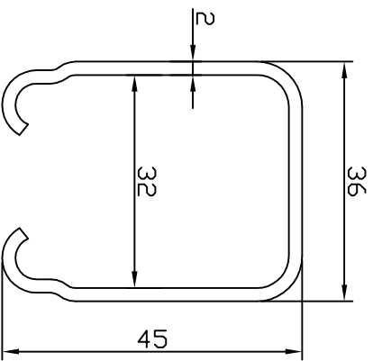
290 Top Track Steel
