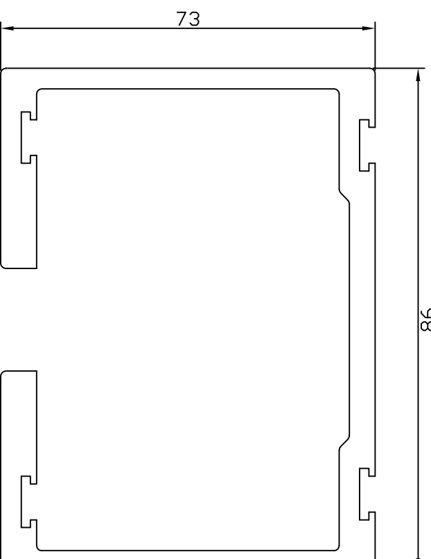
307 Top Track Zinc Plated Steel
