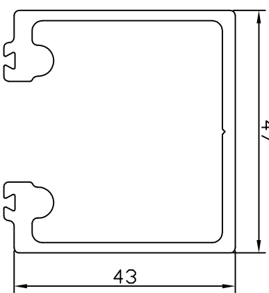
180 Top Track Aluminium
