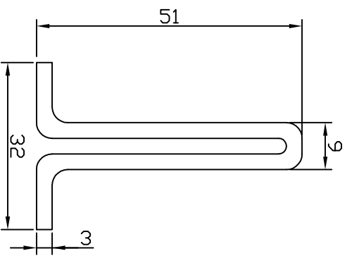
512 Top Guide Channel Aluminum
