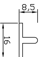
80X Bottom Rail Aluminum
