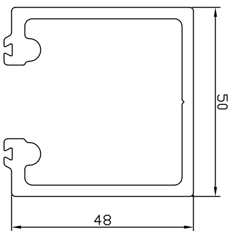
250 Top Track Aluminium
