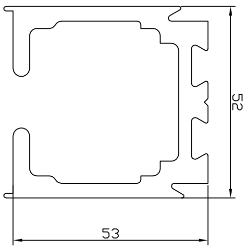
120 Top Track Aluminium
