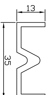
917 Bottom Rail Brass
