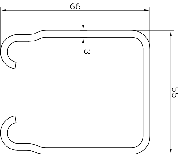
301H Top Track Steel
