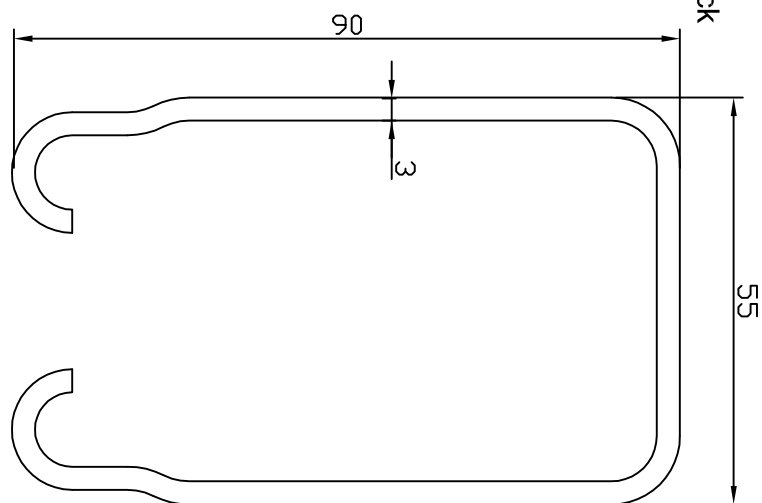
250 Top Track Aluminium
